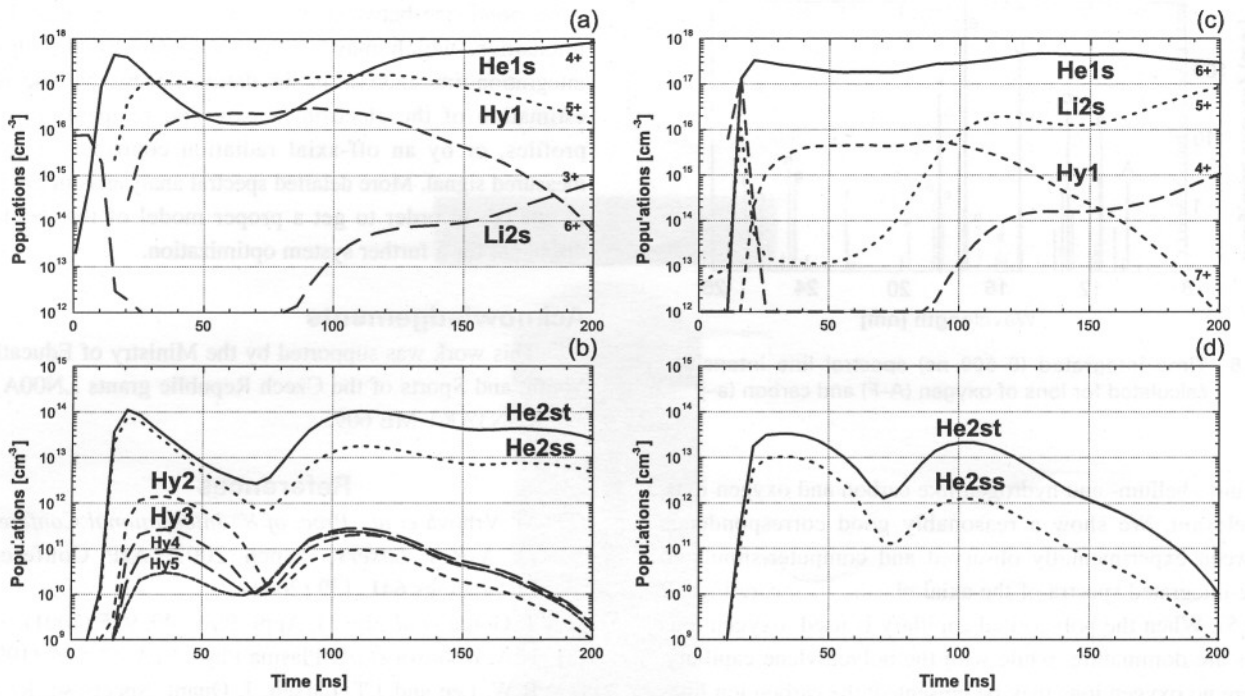
Fig. 4 Time dependences of population densities of (a) carbon ions, (b) excited states of helium- and hydrogen- like carbon ions, (c) oxygen ions, (d) selected excited states of helium- like oxygen ions.
